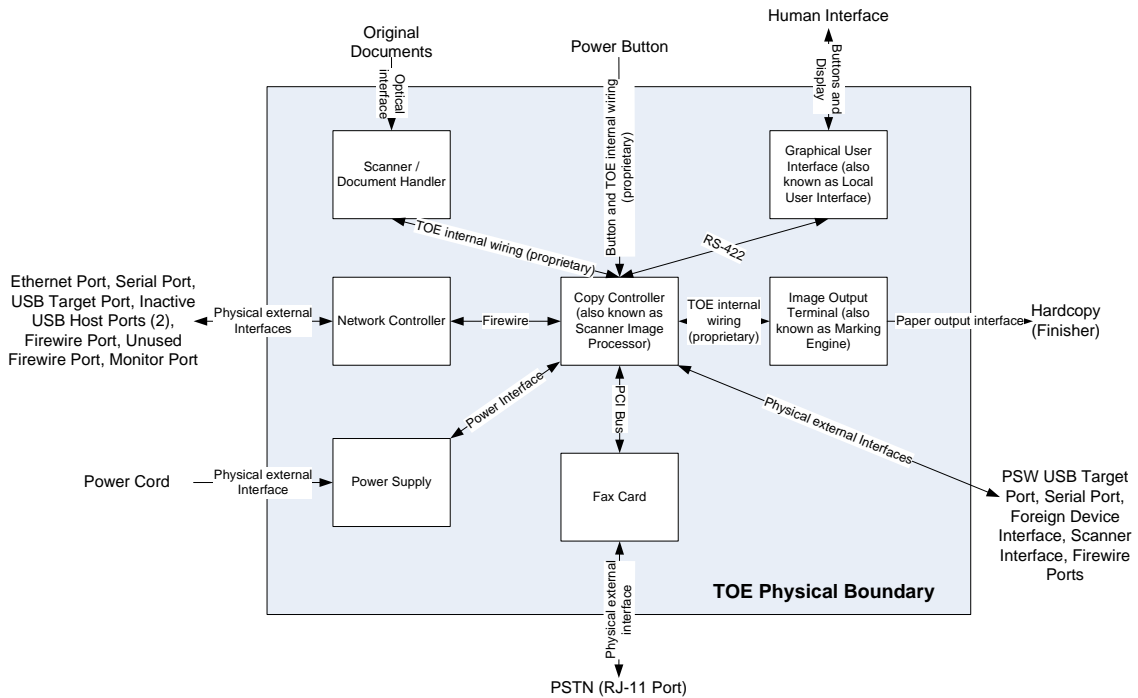
Figure 2-2 TOE System Partitioning, multi-board controller configuration
