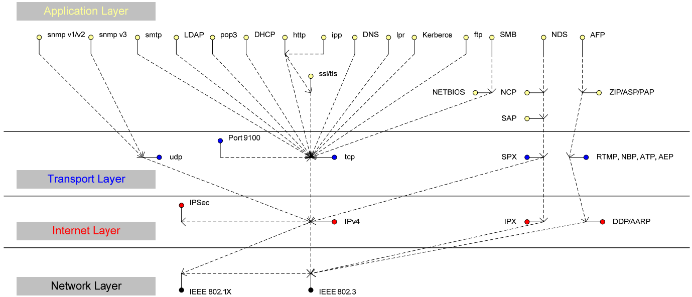
Figure 2-3 Network Controller protocol stacks
