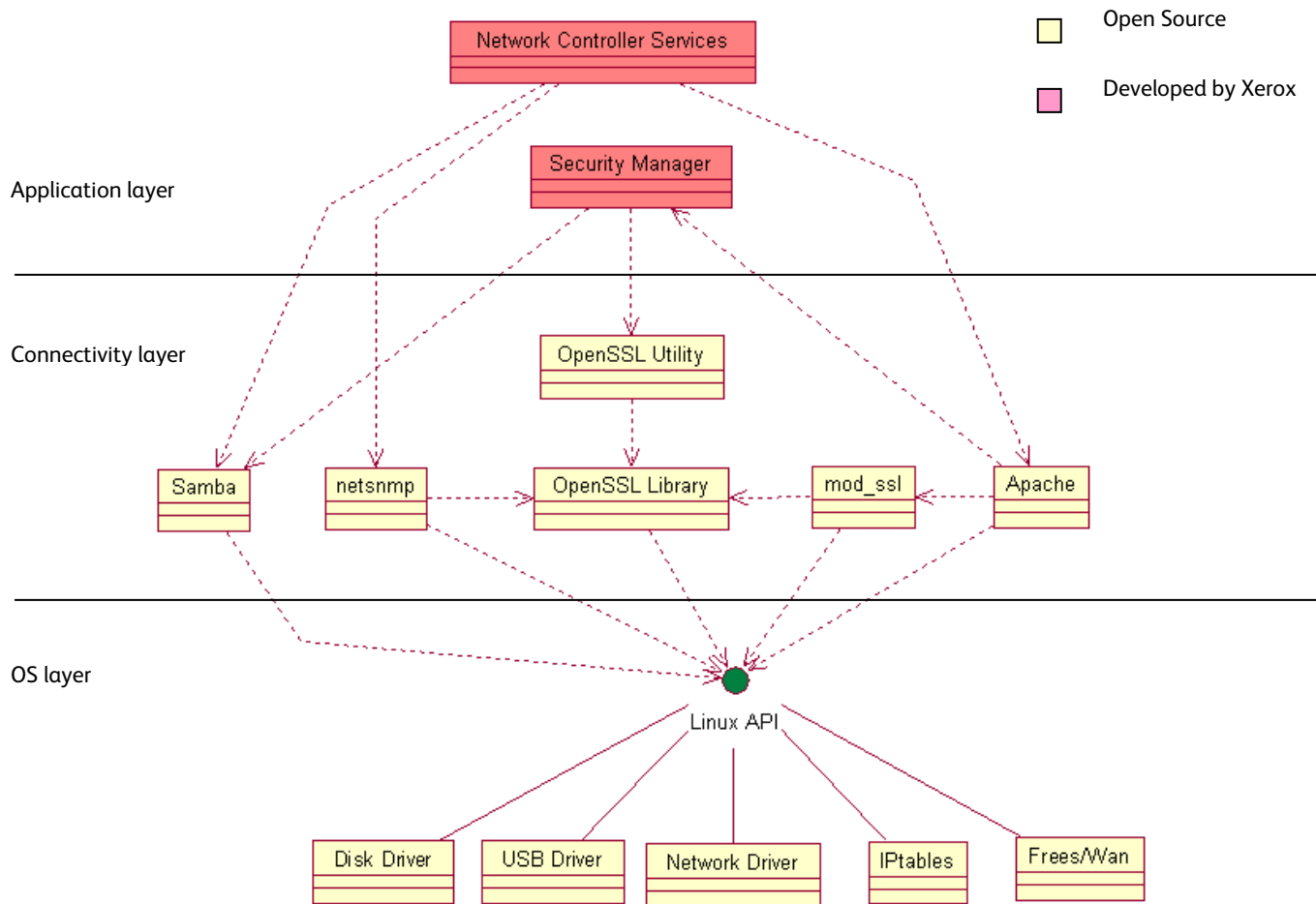
Figure 2-7 Network Controller Operating System layer components
