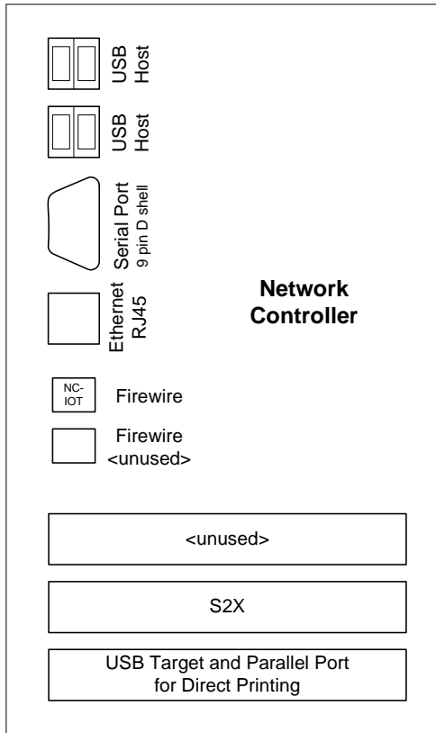
Figure 2-6 Physical Connections located on the Network Controller at lower rear of the machine
