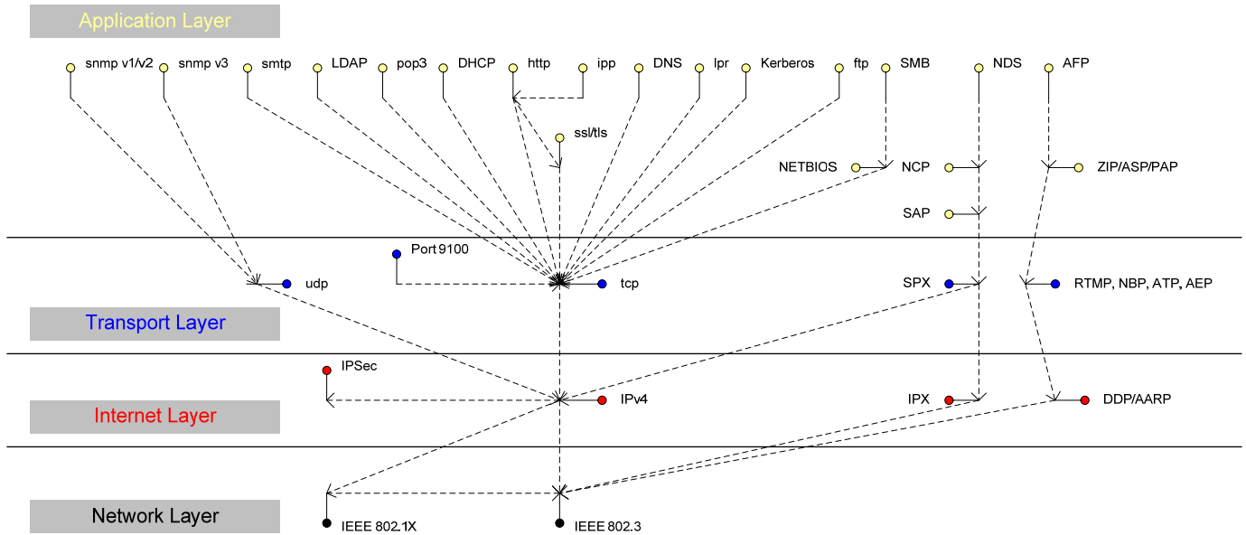
Figure 2-5 Network Controller protocol stacks
