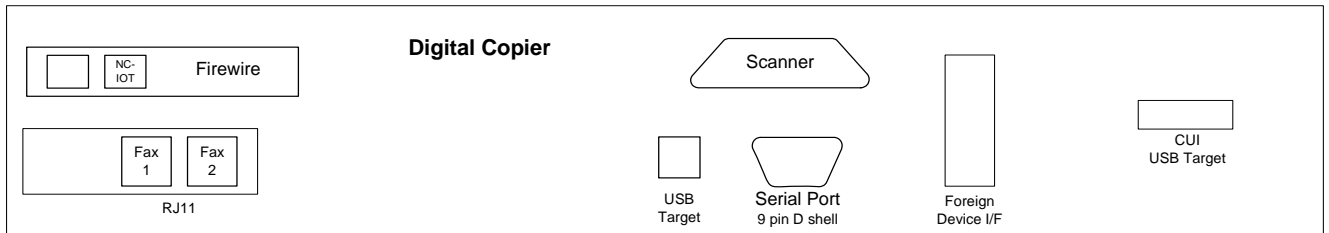
Figure 2-5 Physical Map of Copy Controller external connections [65/75/87 ppm models]
