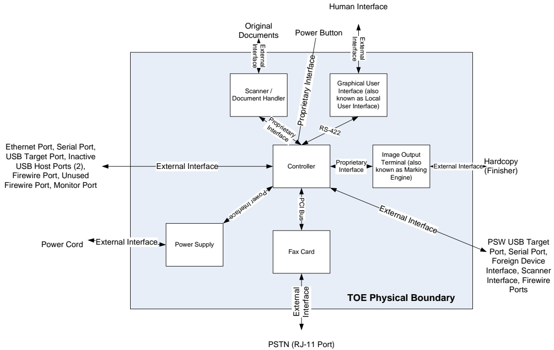
Figure 2-2-3 TOE System Partitioning, single-board Controller configuration (32, 38, 45 and 55ppm models)
