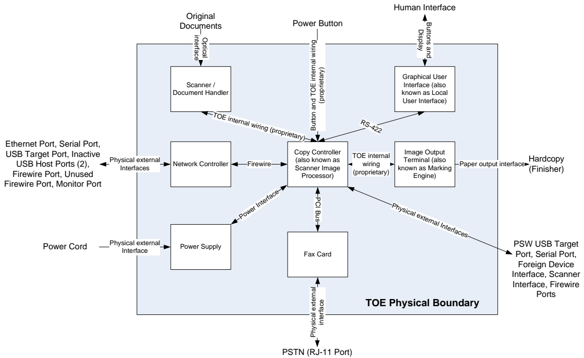
Figure 2-2-2 TOE System Partitioning, multi-board controller configuration (65, 75 and 87 ppm models)
