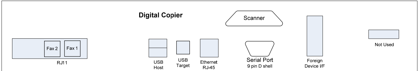
Figure 2-4 Physical Map of Copy Controller external connections [32/38/45/55 ppm models]
