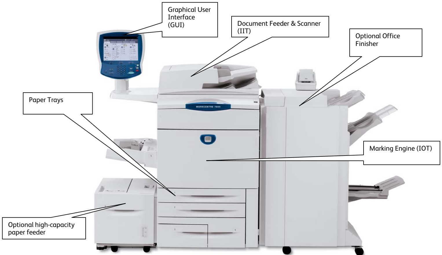
Figure 2-1 WorkCentre Multifunction System
