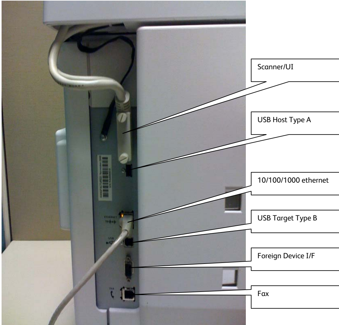
Figure 2-3 Back panel connections
