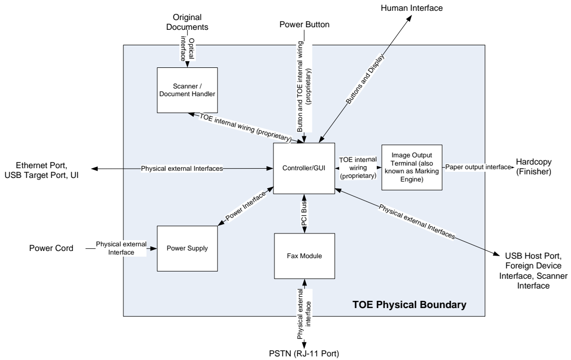
Figure 2-2 System functional block diagram
