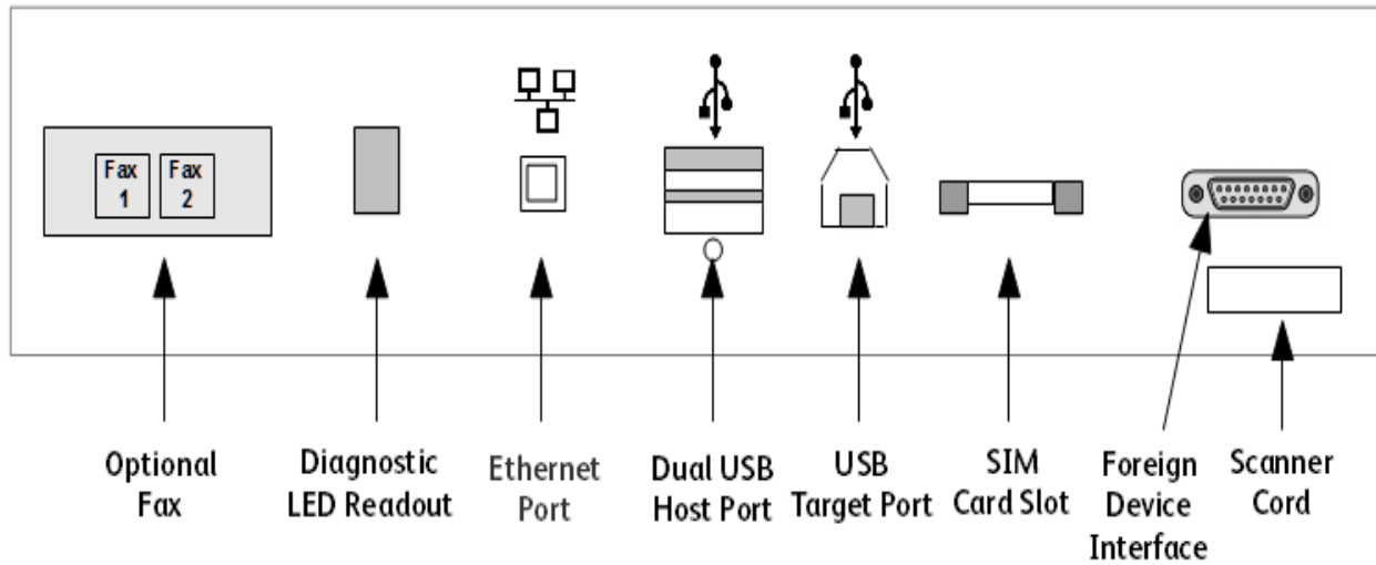
Figure 2-3 WorkCentre 5845/5855/5865/5875/5890 Back panel connections
