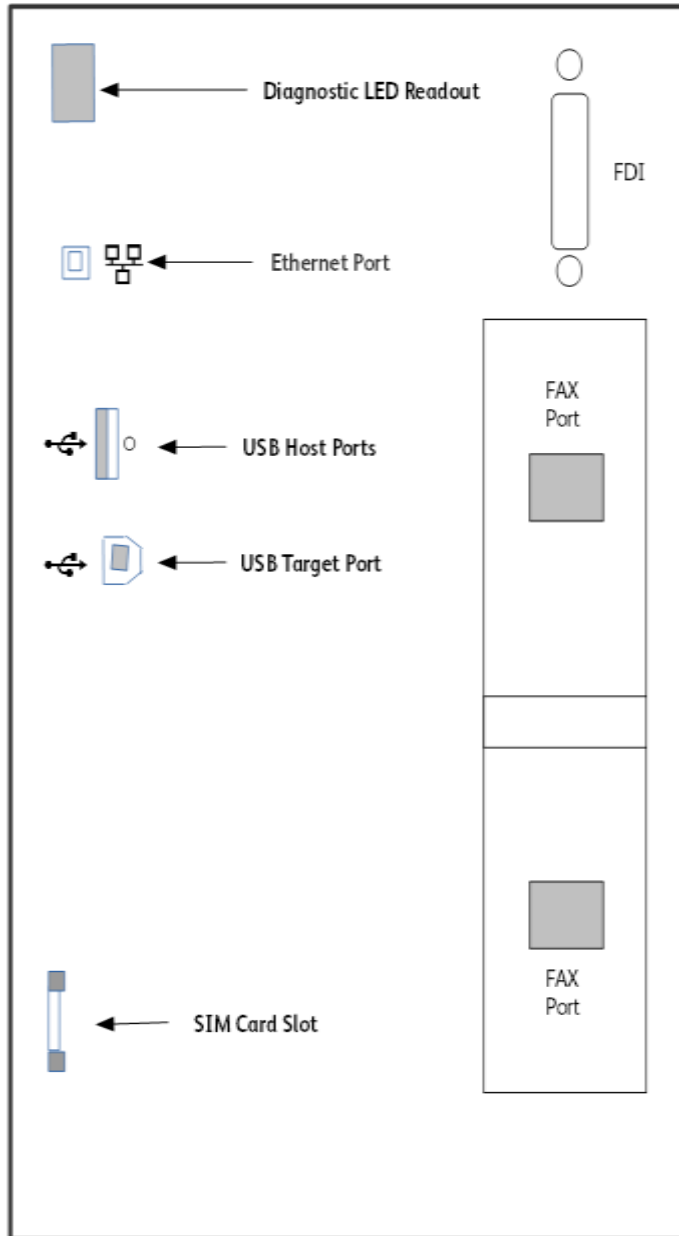
Figure 2-3 WorkCentre 5945/5955 Back panel connections
