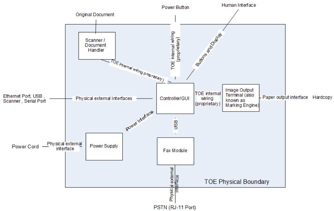
Figure 2-2 System functional block diagram
