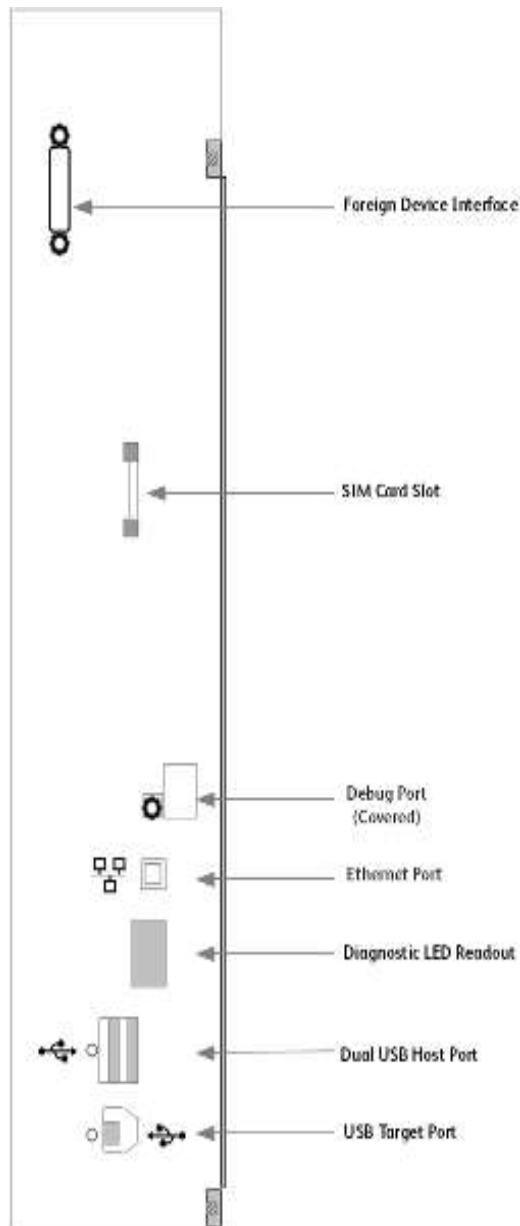
Figure 2-3 WorkCentre 7220-7255 Back panel connections
