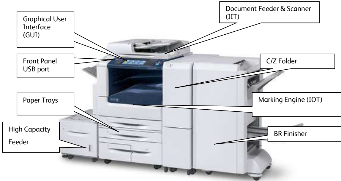
Figure 2-1 WorkCentre 7830/7835/7845/7855 WorkCentre 7970 (shown) Multifunction System
