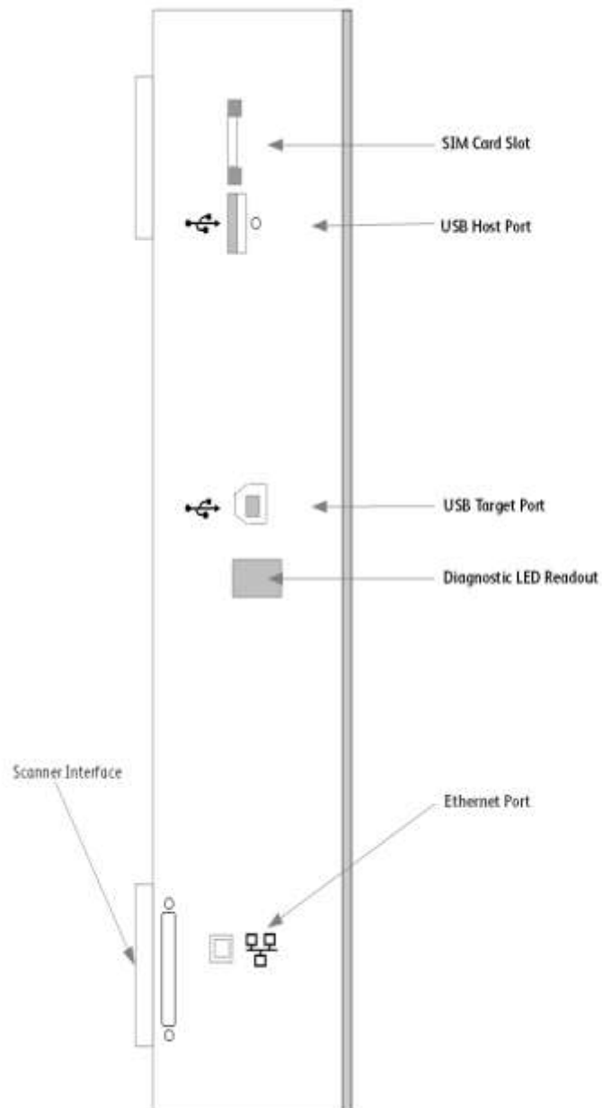
Figure 2-3 WorkCentre 7830/7835/7845/7855 WorkCentre 7970 (shown) Back panel connections
