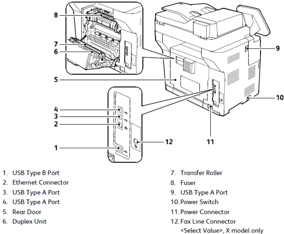
Figure 0-3 WorkCentre 3655i and 3655 Back panel connections
