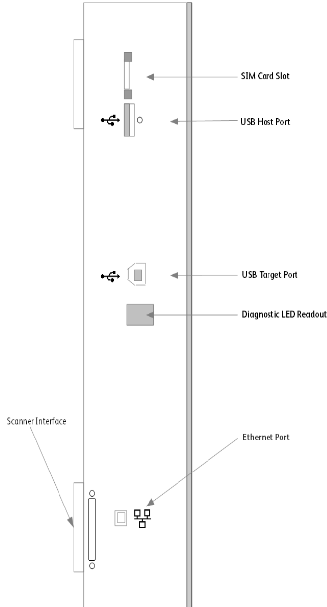
Figure 0-3 WorkCentre 78XXi/78XX Back panel connections
