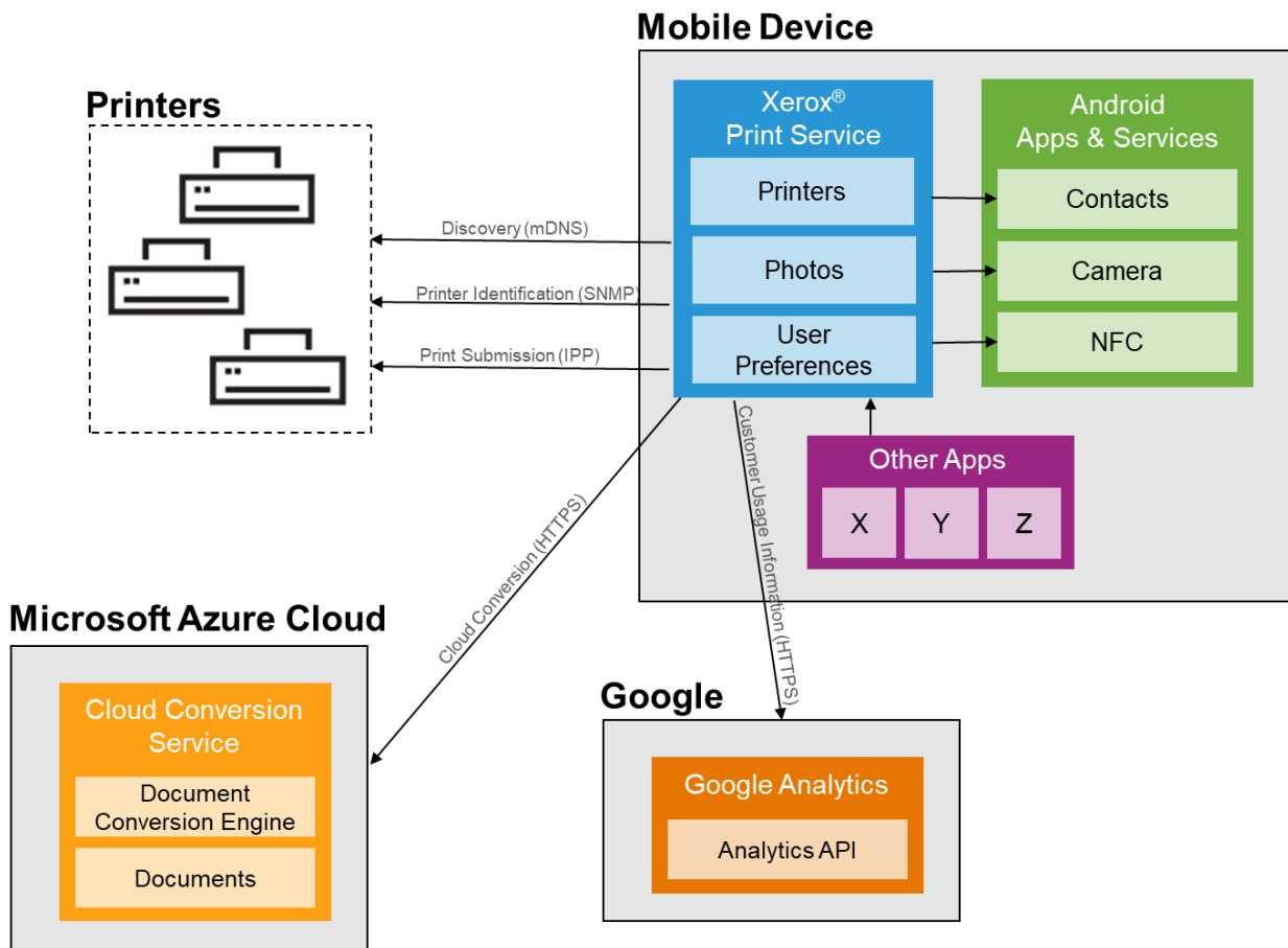
Figure 2.2-1: Component Diagram
