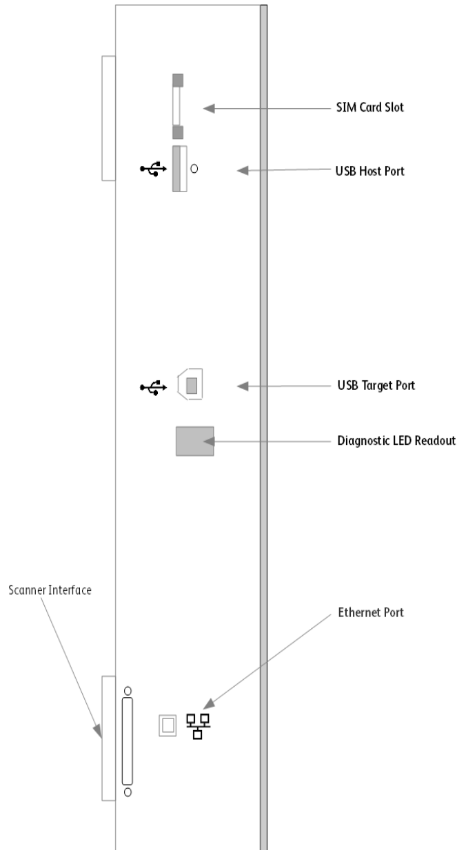
Figure 2-3 EC 7835/7856Back panel connections
