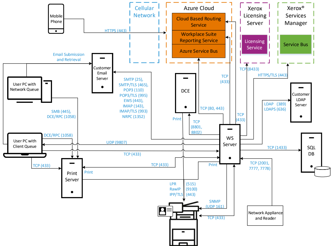
Xerox® Workplace Suite – Network Port Diagram
